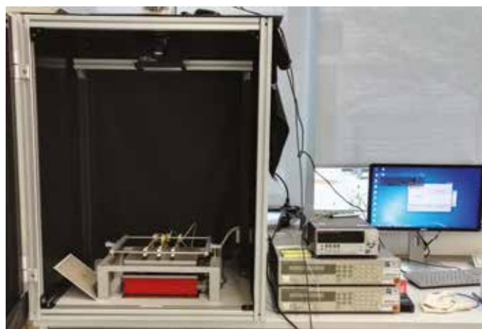
Figure 3. Test set-up of an LED-based light-induced (left) and electrical-induced (right) solar cell LID tester.
